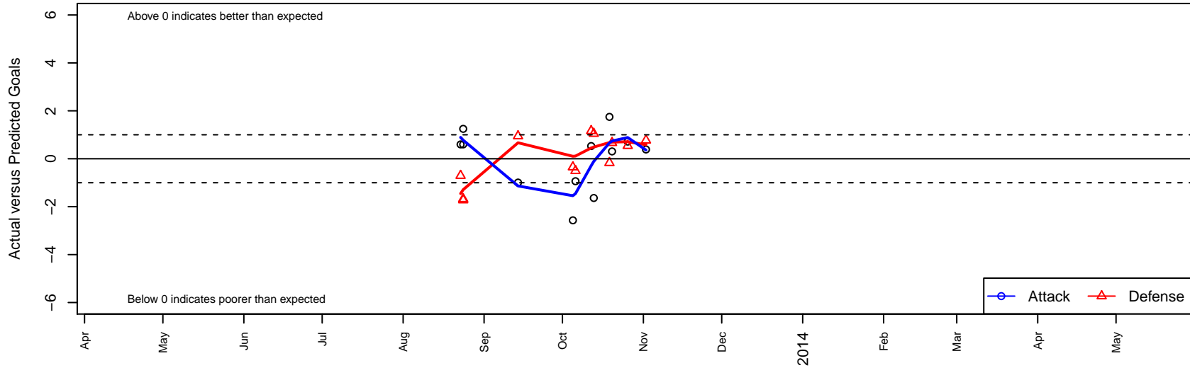
Los Gatos United Panthers B01 Dots are actual minus expected GF (blue circles) and GA (red triangles). Blue line is smoothed change in attack strength. Red is smoothed change in defense strength.
